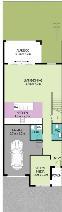
GROUND FLOOR
